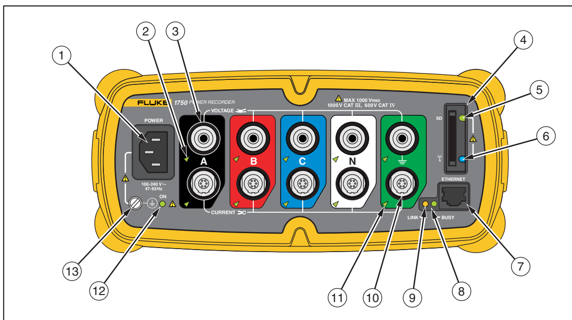
Figura 1. Power Recorder 1750 de Fluke
